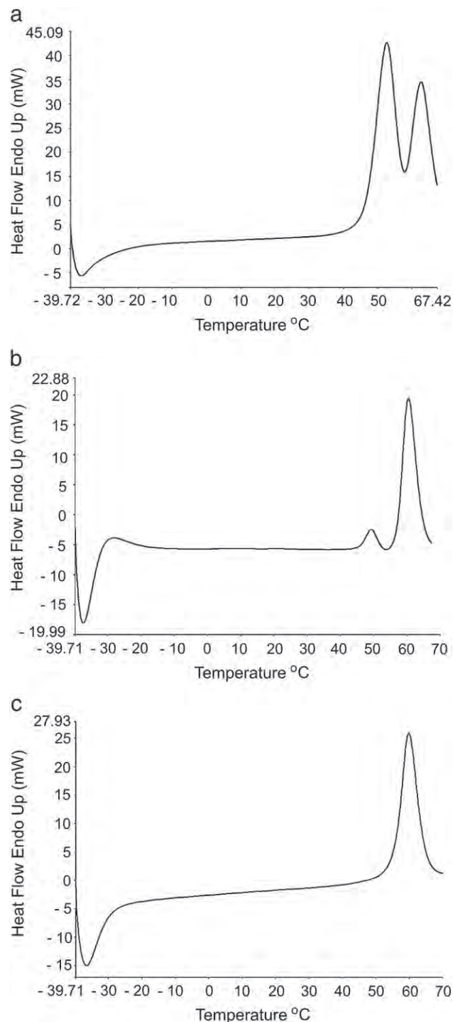
Fig. 9. DSC scans of sample Y1 from a) untreated b) lightly ground and c) more heavily ground material obtained at 100 \text{ °C min}^{-1} .
